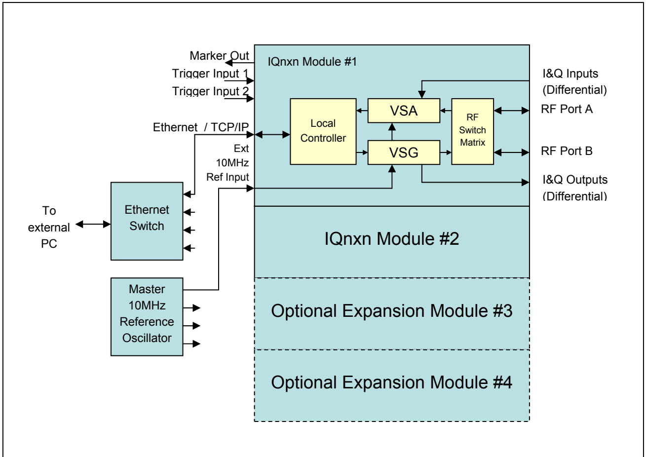
Figure 4. Basic block diagram of the IQnxxn instrument
